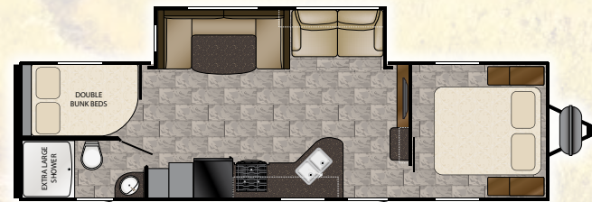
TR 29 MSB Length: 34' 1" Dry: 6,998 Height: 11' 2" Hitch: 770 Tanks: 42 F 35 G 35 B
