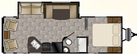
TR 25 RL Length: 29' 6" Dry: 6,151 Height: 11' 2" Hitch: 642 Tanks: 42 F 35 G 35 B
