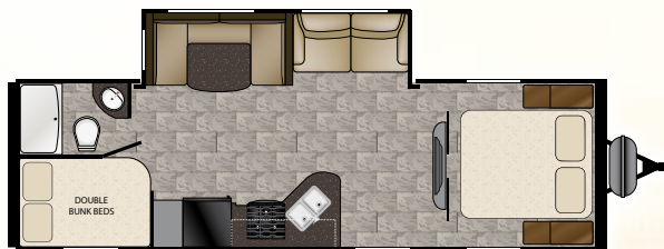
TR 27 FQBS Length: 30' 7" Dry: 6,081 Height: 11' 2" Hitch: 725 Tanks: 42 F 35 G 35 B
